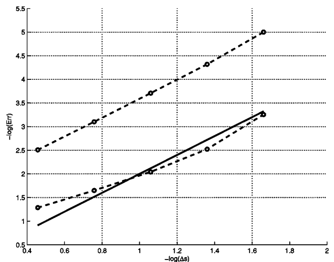
FIG. 4. Log-log plot of the discretization error in the computation of the velocity field due to a translating sphere. The two dashed lines show the error at two different locations in space. The regularization parameter was fixed at \epsilon = 0.01 . The solid line has slope two, indicating a discretization error O(\Delta s^2) for small values of \Delta s = \Delta s_1 = \Delta s_2 (large abscissa values).
